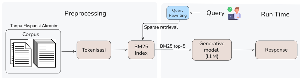
Gambar IV.6 Diagram Alur Pipeline Konfigurasi BM25 + Query Rewriting
